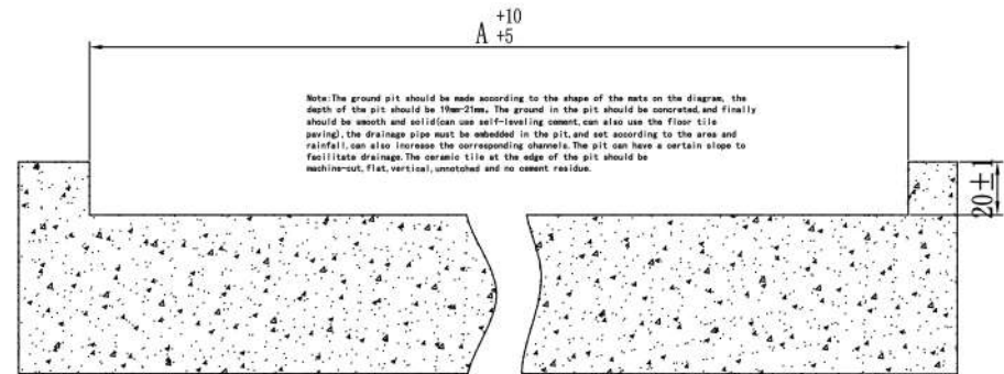
X-X Section view of pit
